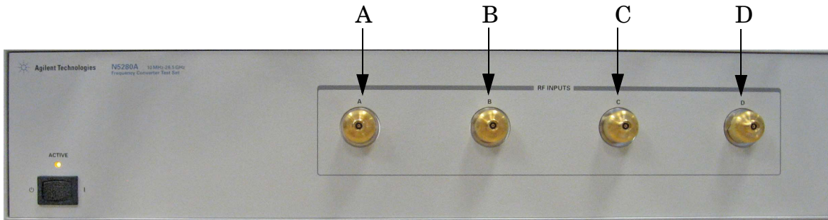
Figure 5 Front Panel
