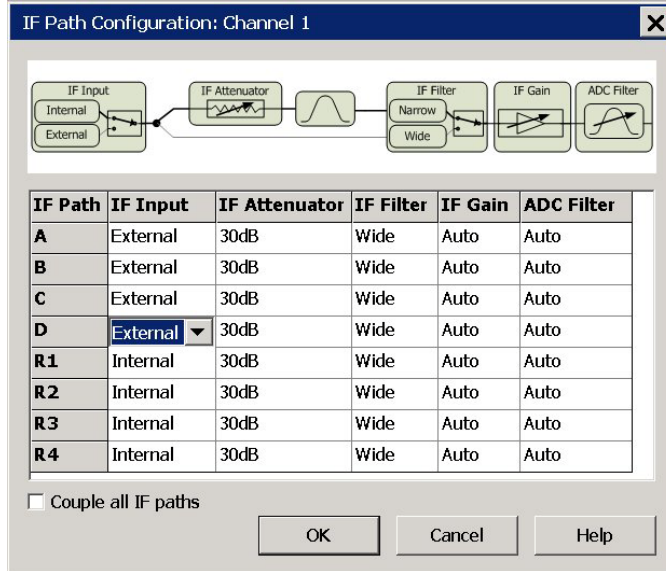
Figure 17 IF Input
